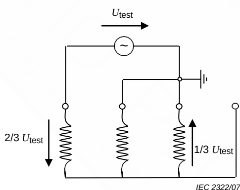
Figure 4 – Phase-to-earth test circuit for single-phase excitation
