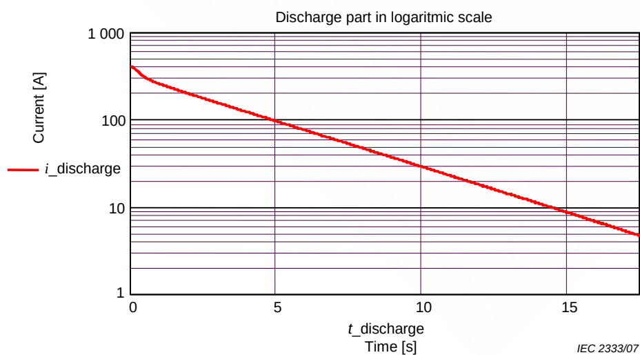
Figure B.4a – Graph of the charge and discharge current
